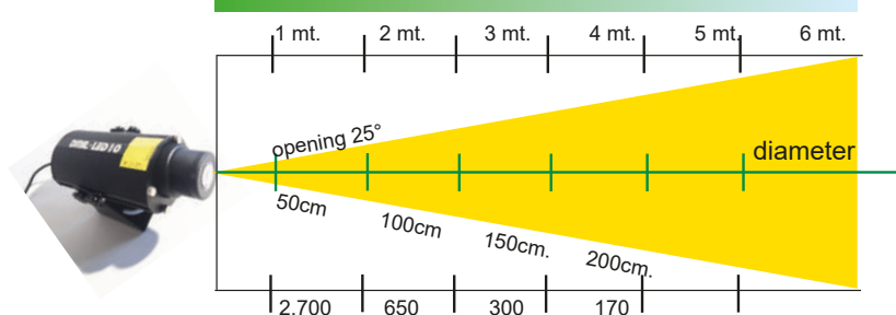
Example image aperture at different distances with 25° aperture focal length
