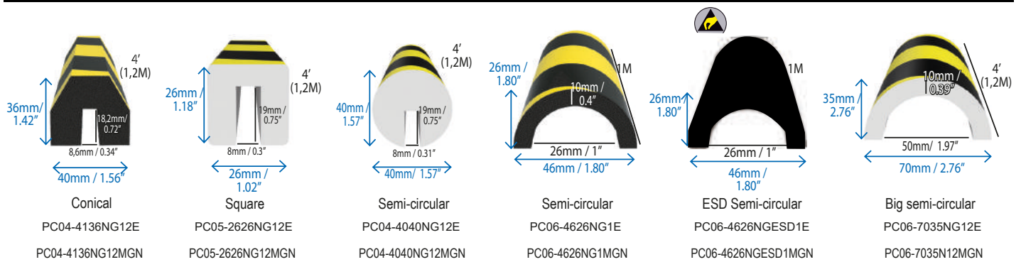
Tubular protections or with L-shaped beams
